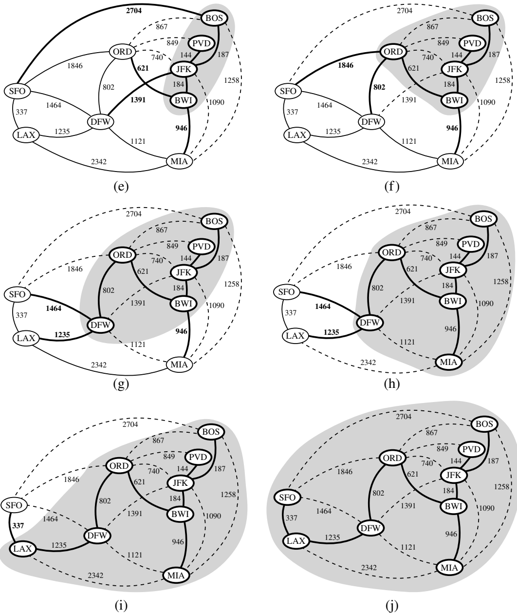
Figure 14.21: An illustration of the Prim-Jarnik MST algorithm. (Continued from Figure 14.20.)
